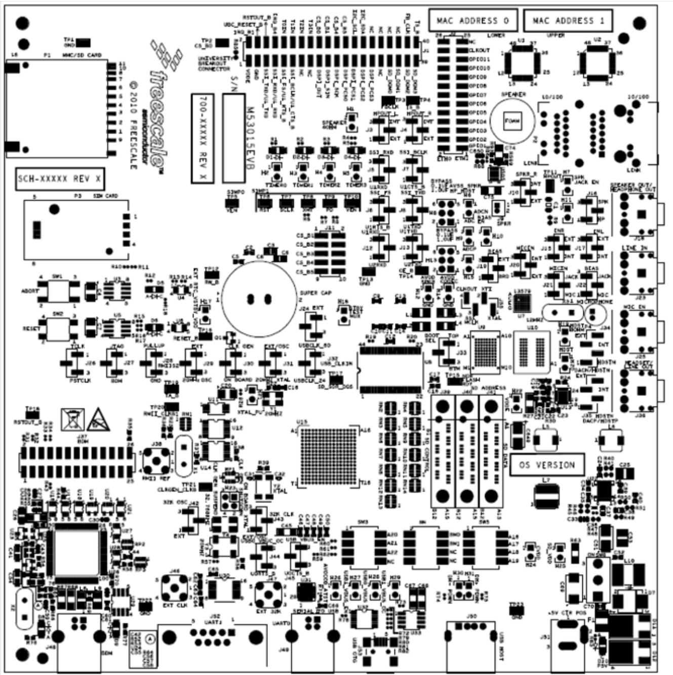
Figure 2. Board Diagram
