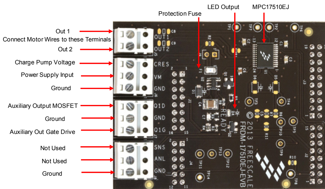
Figure 2. Board Description
