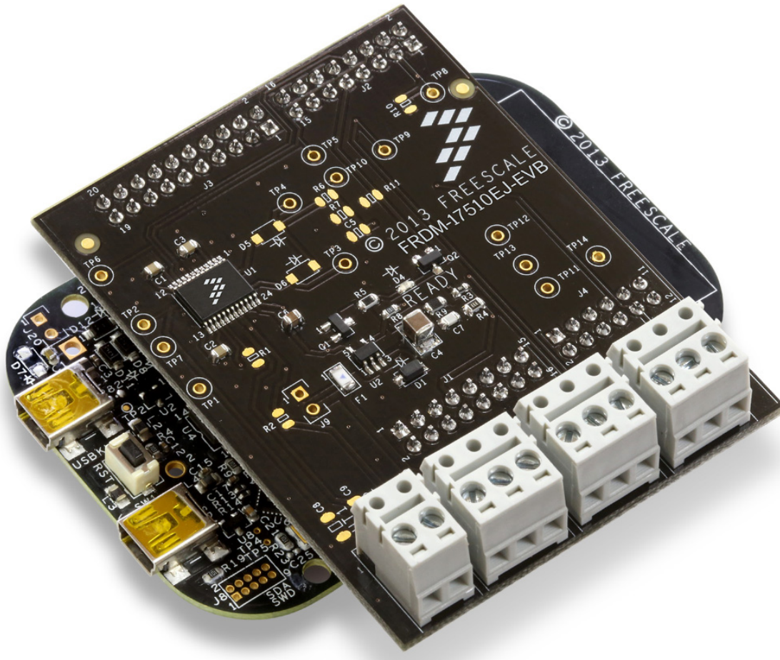
Figure 1. FRDM-17510EJ-EVB Evaluation Board
