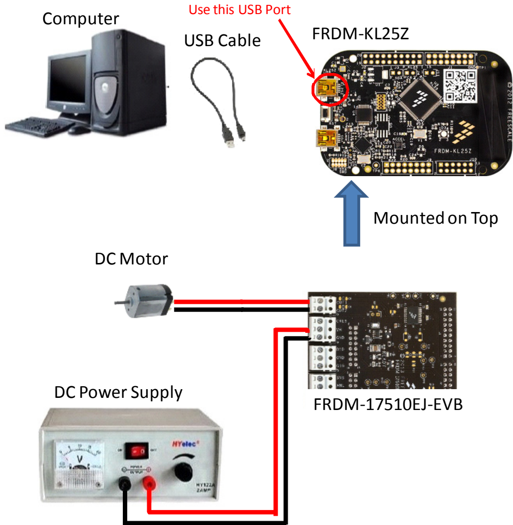
Figure 5. FRDM-17510EJ-EVB Plus FRDM-KL25Z Board Setup
